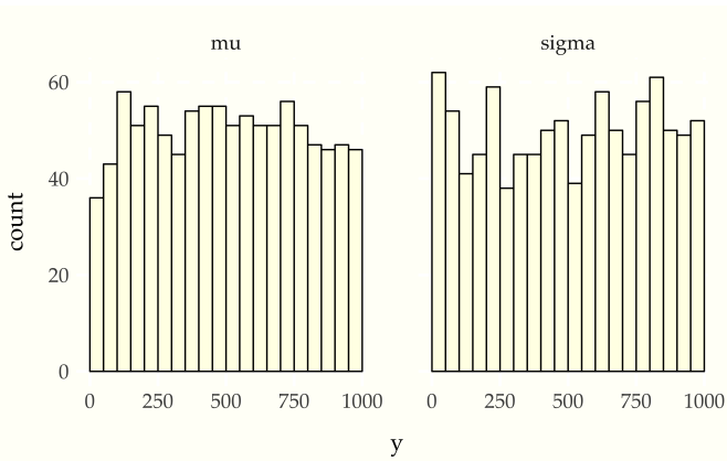
Figure 28.1: Simulation based calibration plots for location and scale of a normal model with standard normal prior on the location standard lognormal prior on the scale. Both histograms appear uniform, which is consistent with inference being well calibrated.
