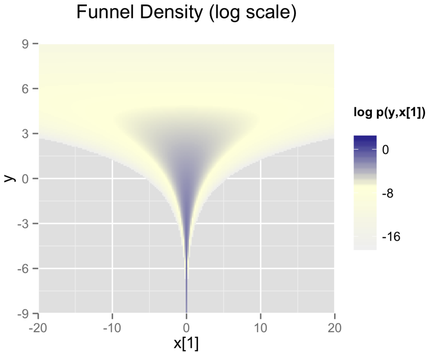
Figure 21.1: Neal's funnel density
